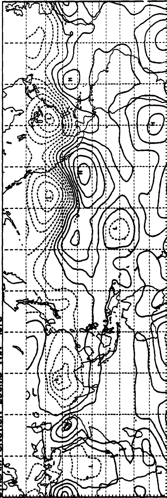
STREAM FUNCTION 200MB WIN 1978
